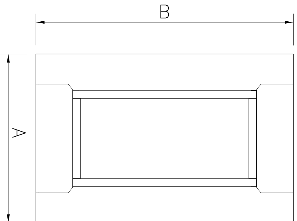
TOP VIEW
